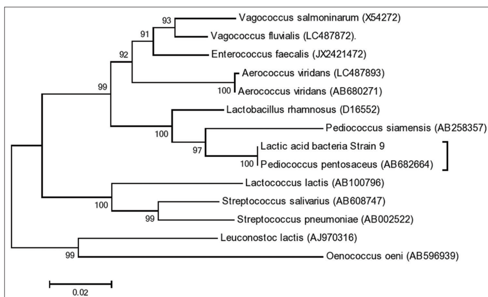
Figure-1: Phylogenetic tree constructed using the neighbor-joining algorithm of 16S rRNA gene nucleotides sequence. The number in each phylogram branch indicates a bootstrap value (%) by 1000-replication multiple, and scale shows two per 100 nucleotide substitutions.
