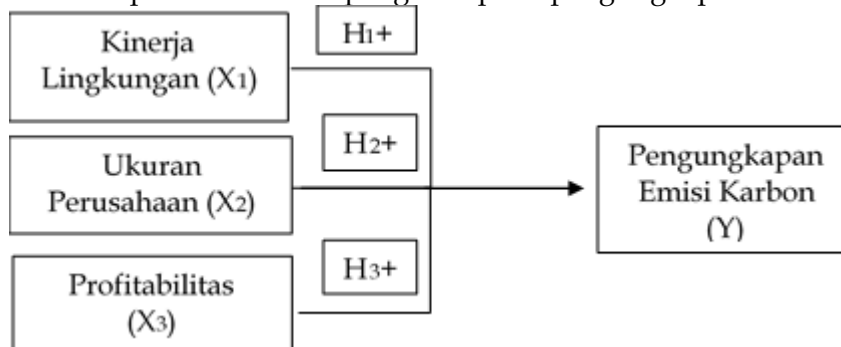
Gambar 1. Model Penelitian
