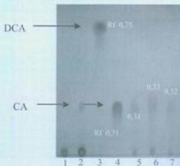
Gambar 1. Transformasi CA oleh Lactobacillus spp. isolat susu kambing etawa. (1) MRS broth, (2) MRS broth ditambahkan dengan CA, (3) asam deoksikolat (DCA), (4) asam kolat (CA), (5) Lactobacillus sp. GMA46, (6) Lactobacillus sp. GMA47, (7) Lactobacillus sp. GMA50
