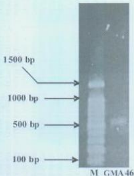
Gambar 2. Hasil PCR 16S rDNA Lactobacillus sp. GMA46 isolat susu kambing etawa pada agarosa 1,2%. Keterangan: (M) marker (1) Lactobacillus sp. GMA46
