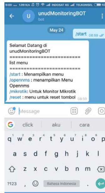
Gambar 6 Menu start
