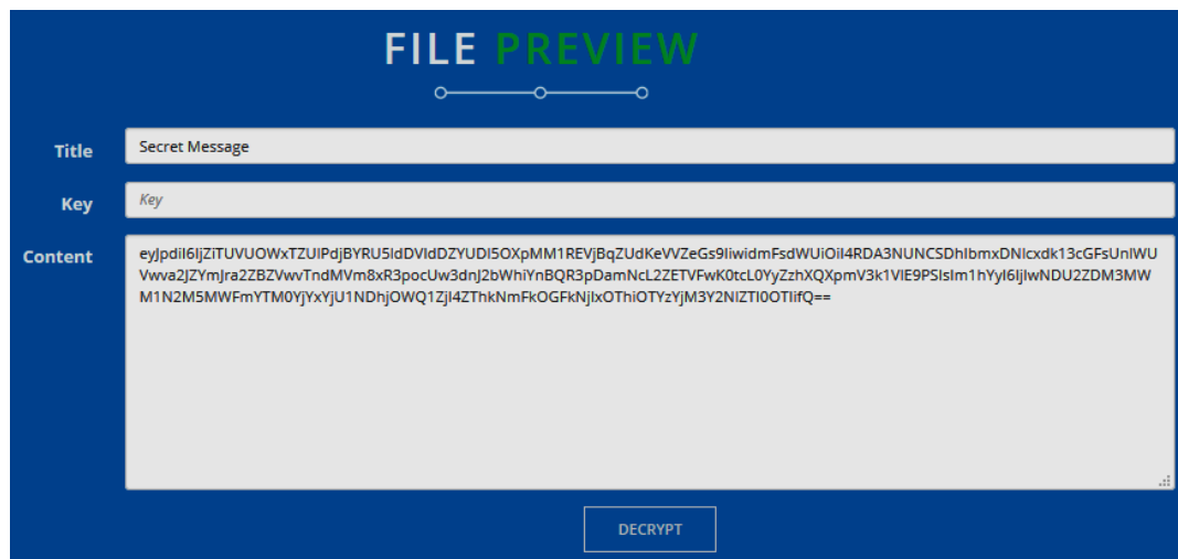
Figure 5. Chypertext File
