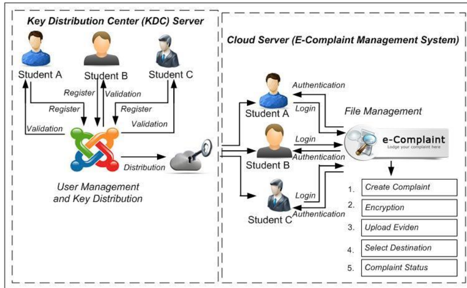
Figure 3. Applied Anonymous Authentication for Complain System
