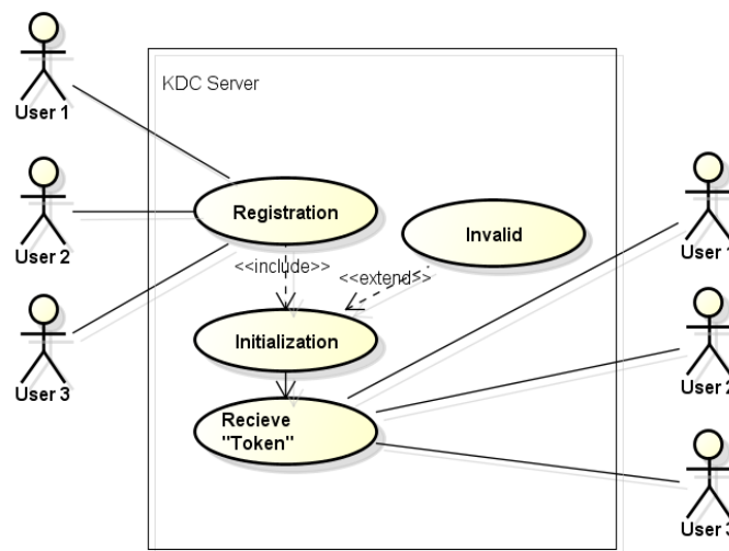
Figure 1. Use Case Diagram KDC Server
