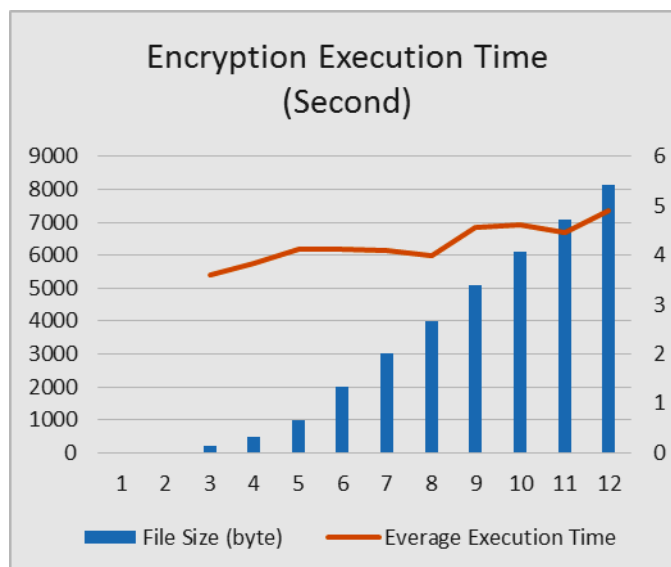
Figure 16. Performance of ABE Algorithm
