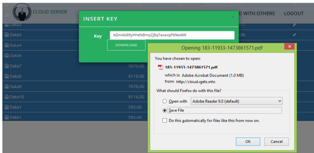
Figure 12. Downloaded File
