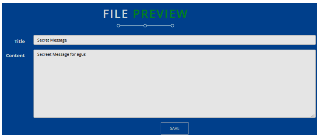
Figure 8. Plaintext File
