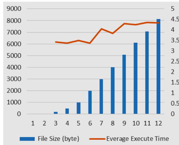
Figure 17. Performance of ABS Algorithm (in Seconds)
