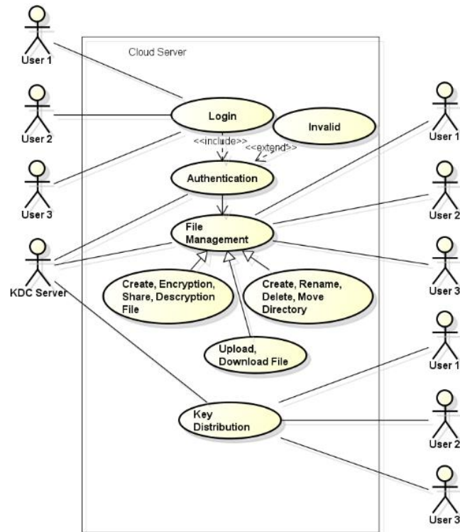
Figure 2. User Case Diagram Cloud Server
