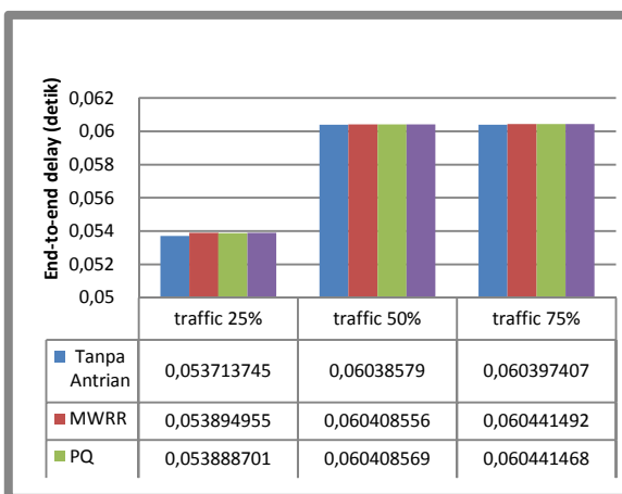
Gambar 4. Grafik rata-rata end-to-end delay
