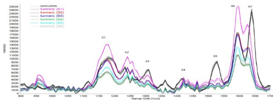
Figure 1. Raman spectra of curcumin and turmeric rhizome
